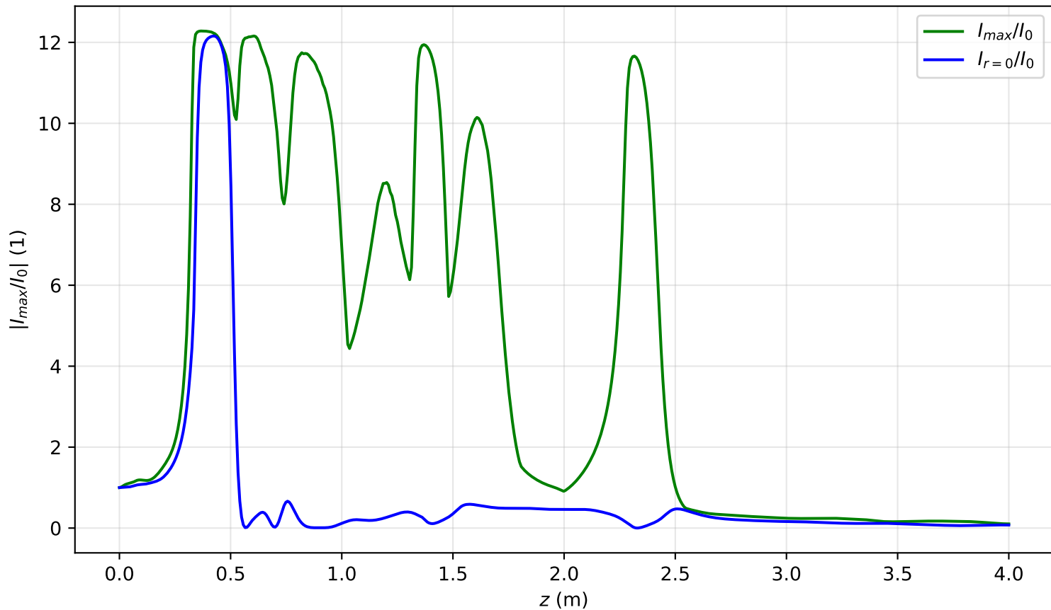
I_{max}(x=0, y=0, z)/I_0 , Pin=9.0Pcr, noisy input, artificial time
